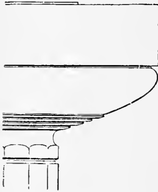
FIG. 53.—GREEK DORIC CAPITAL FROM SELINUS.
